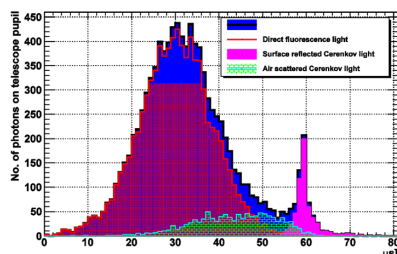
Example of the signal generated by an UHECR on the JEM-EUSO focal surface.
