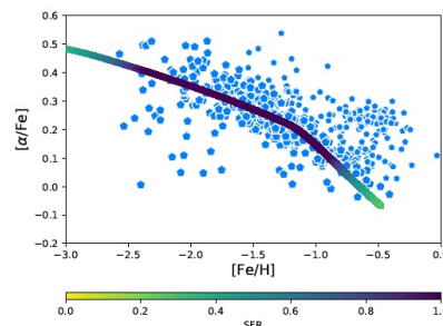
[\alpha/Fe] as a function of [Fe/H] . The cyan pentagons are stars measured by APOGEE, which belong to Gaia-Enceladus. The model is shown as a line and it is colourcoded according to the SFR (see colorbar).
